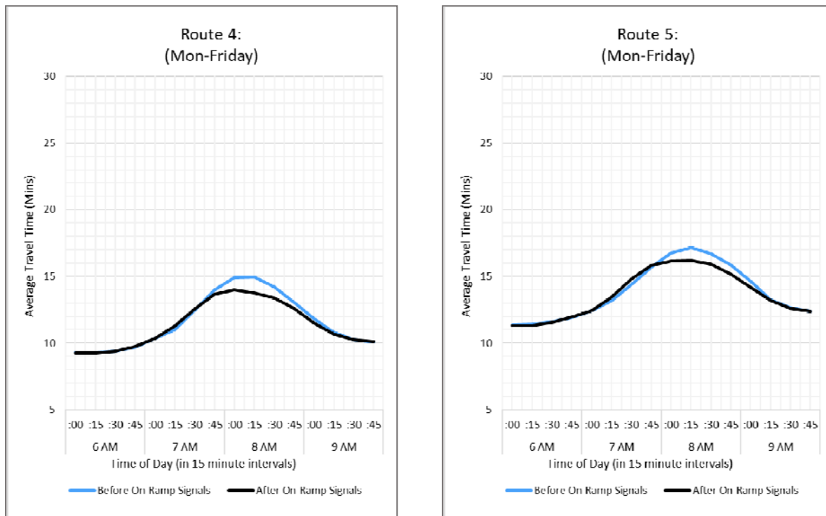
Exhibit 20: Travel Time Comparison for Route 4 (Six Forks Rd. at Norwood) and Route 5 (Six Forks Rd. at Spring Forest)
