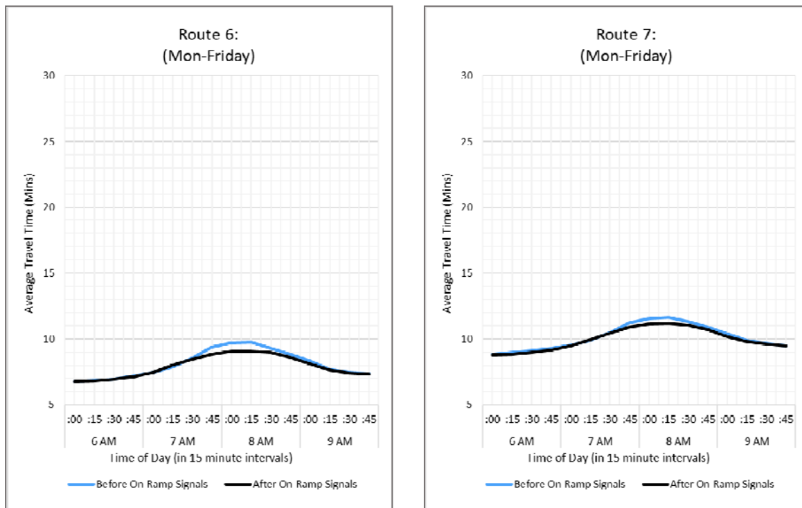
Exhibit 21: Travel Time Comparison for Route 6 (Creedmoor Rd. at Norwood) and Route 7 (Creedmoor Rd. at Lynn)
