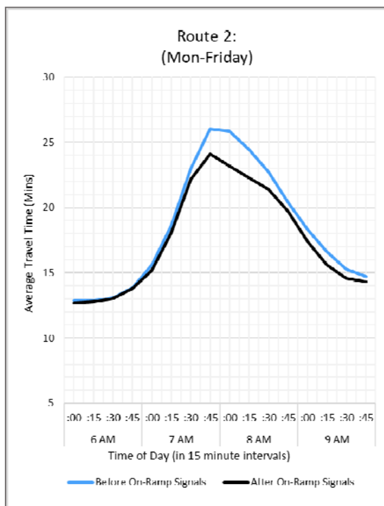
Exhibit 19: Travel Time Comparison for Route 2 (Falls of Neuse Rd. at New Falls) and Route 3 (Falls of Neuse Rd. at Spring Forest)
